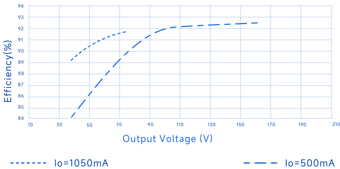
Efficiency Vs. Output Voltage (Vin=230Vac)
