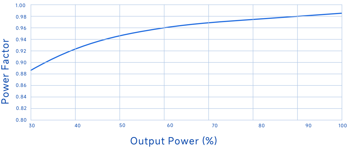
Power Factor Vs. Output Power(Vin=230Vac)
