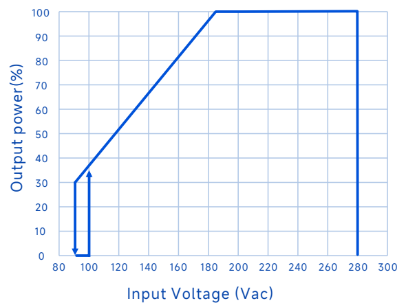
ACI Dimming Curve
