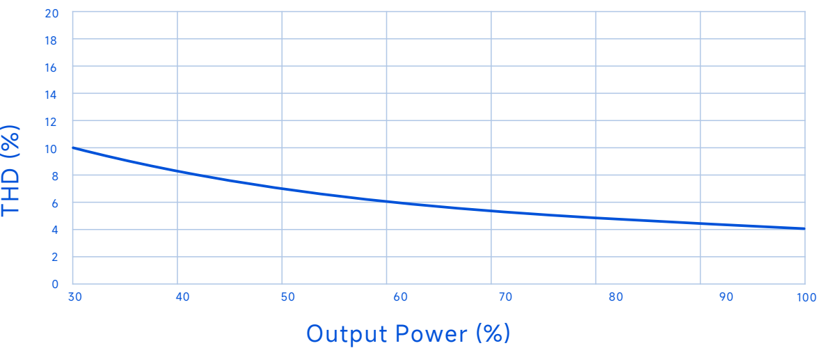
THD Vs. Output Power(Vin=230Vac)
